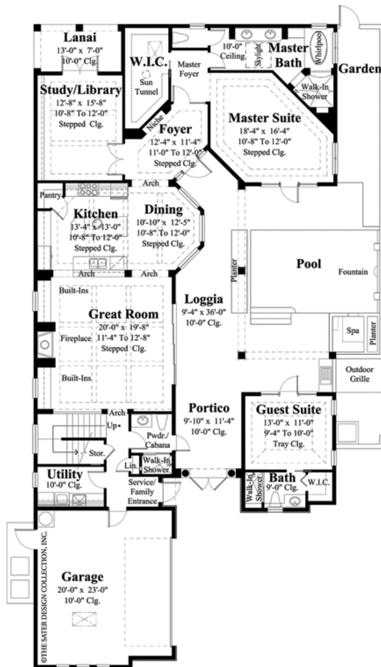
Main Floor
